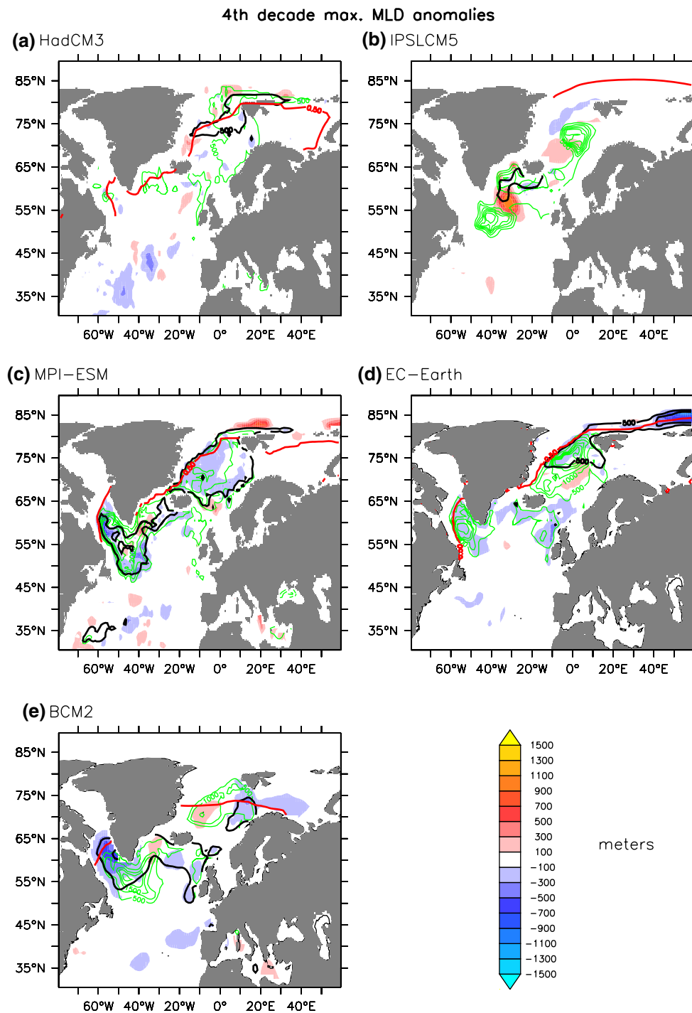
Fig. 3 Differences in the annual maximum of the mixed layer depth between FutHos and FutCon experiments averaged over the 4th decade (2080–2089) for the different models (unit: meter). Black contoured lines are annual maximum of the mixed layer depth over the period 2050–2089 in the FutCon experiments and the green contour
