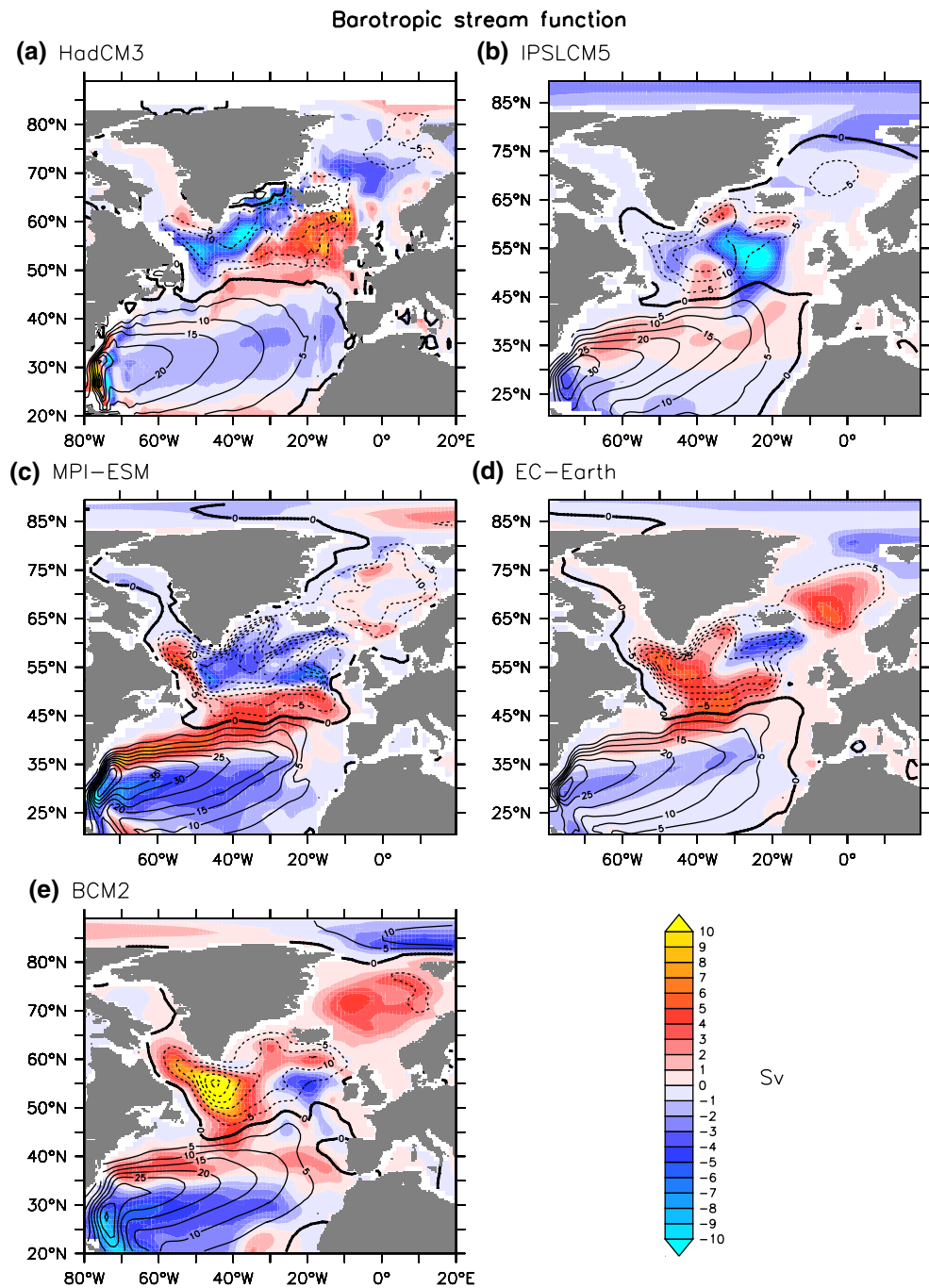
Fig. 14 Difference in barotropic stream function between control projection (FutCon, 2050–2089) and control historical (HisCon, 1965–2004) experiments averaged over the four decades for the different models (unit: Sv). Contoured lines are the barotropic stream function averaged over the period 1964–2004 in the control historical simulations (HisCon, convention for the lines as above). a HadCM3, b IPSLCM5, c MPI-ESM, d EC-Earth and e BCM2. The colour interval is 1 Sv and the contour line interval is 5 Sv
