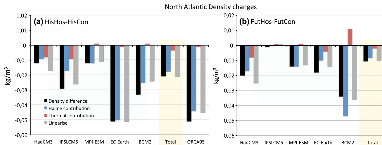
Fig. 10 North Atlantic density changes averaged over the whole column for the last decade a HisHos-HisCon and b (FutHos-FutCon). A linearization of density with respect to salinity and temperature has been done. The blue and red bars correspond to the haline and thermal components respectively, while the black line is the total density
