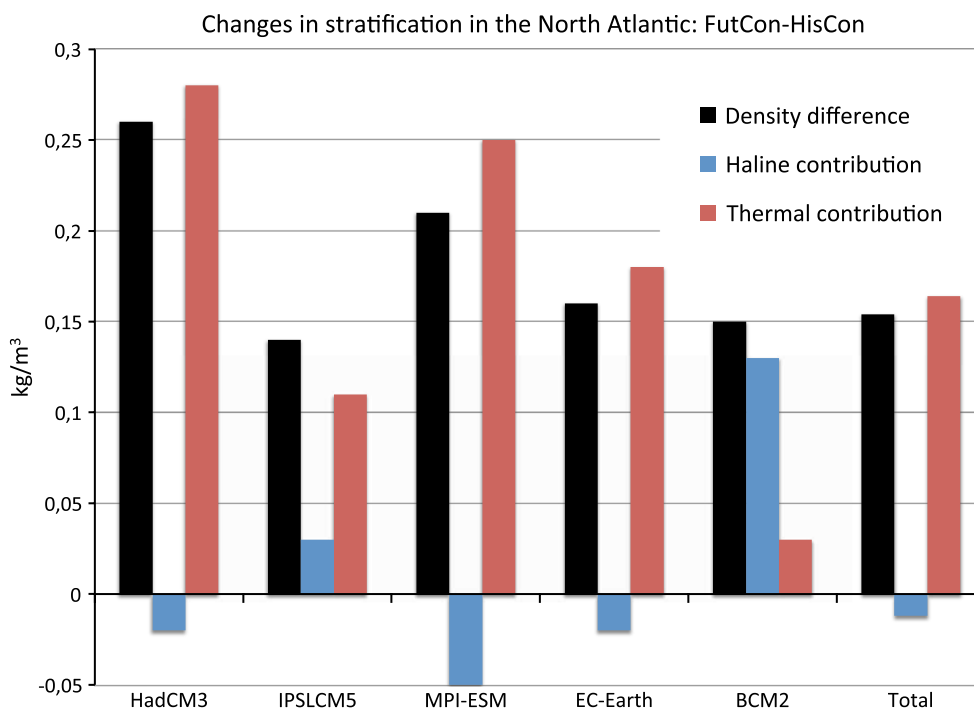
Fig. 5 Density differences between historical and RCP8.5 for the top 1,000 m minus density below 1,000 m averaged over the North Atlantic region (70°E–20°W; 45°N–80°N) as represent in Fig. 2 for the different models and the ensemble mean (column total). A linearization
