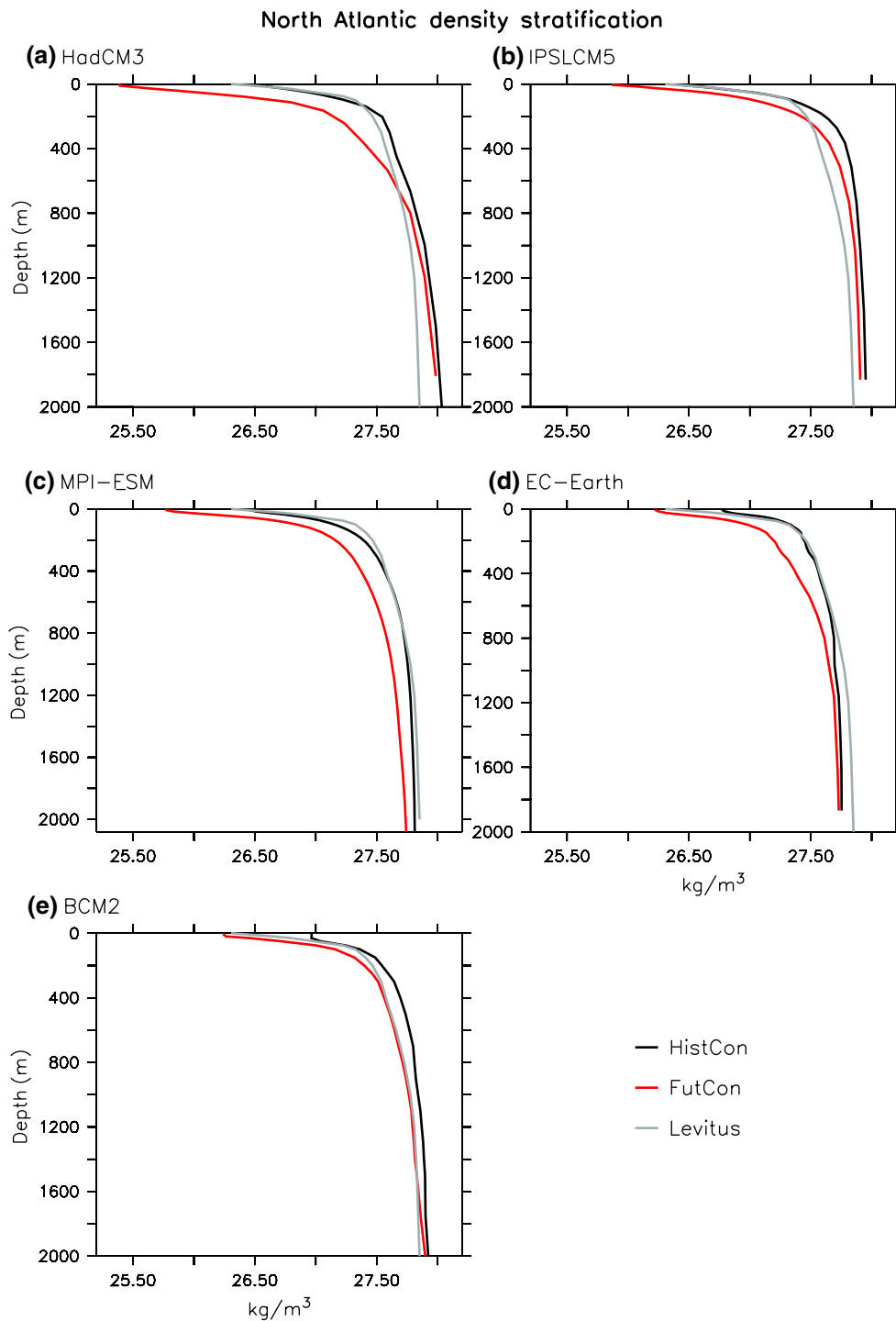
Fig. 2 Density profiles in the historical (HisCon) and projection simulations (FutCon) in standard configuration (i.e. without additional FW hosing) averaged over 40 years of simulations (1965–2004 for historical and 2050–2089 for projection simulations) and for the Lev-
