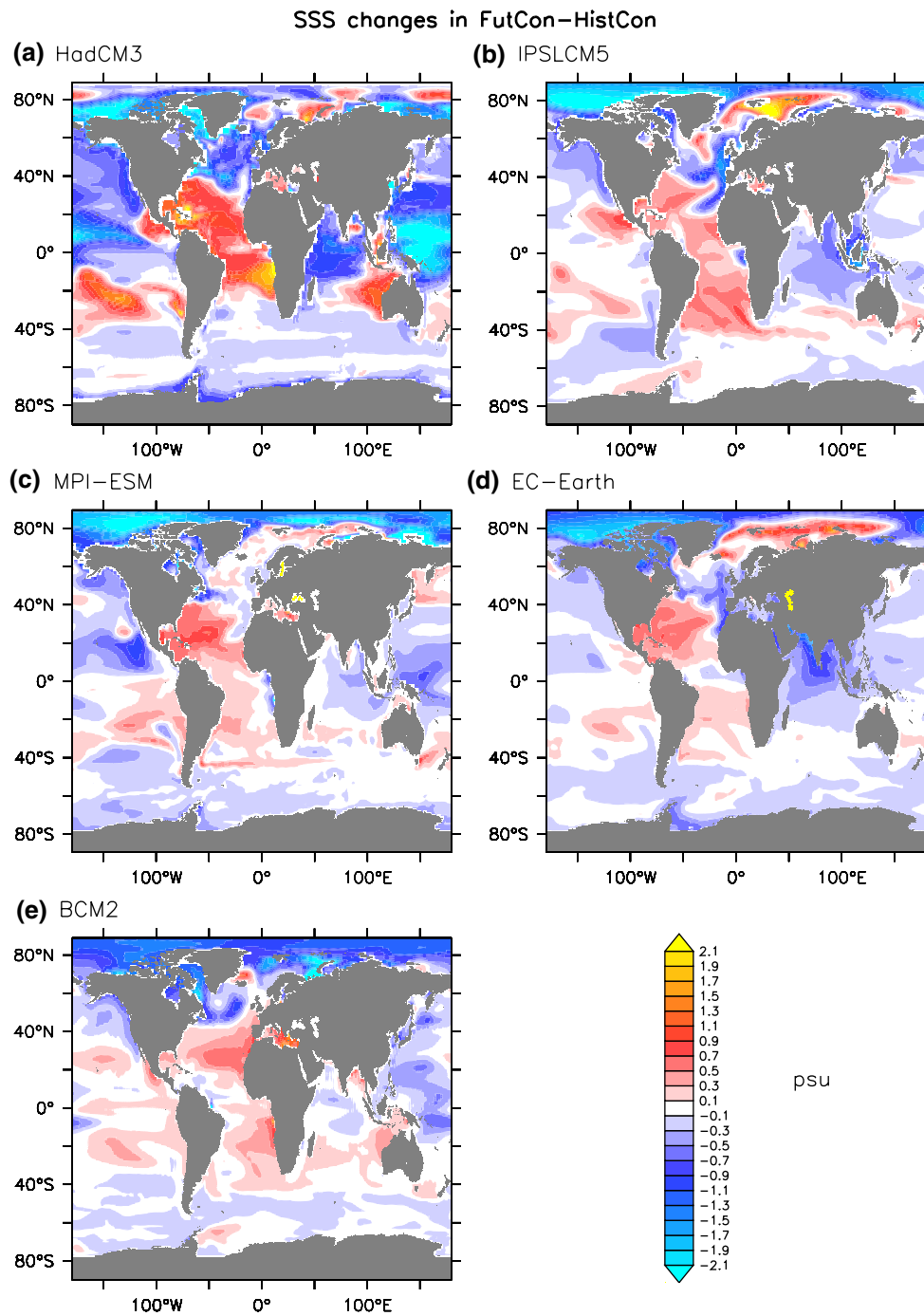
Fig. 6 Sea surface salinity (SSS) changes in the different projections without GrIS melting averaged over the years 2050–2089 as compared to SSS in historical simulations averaged over years 1965–2004
