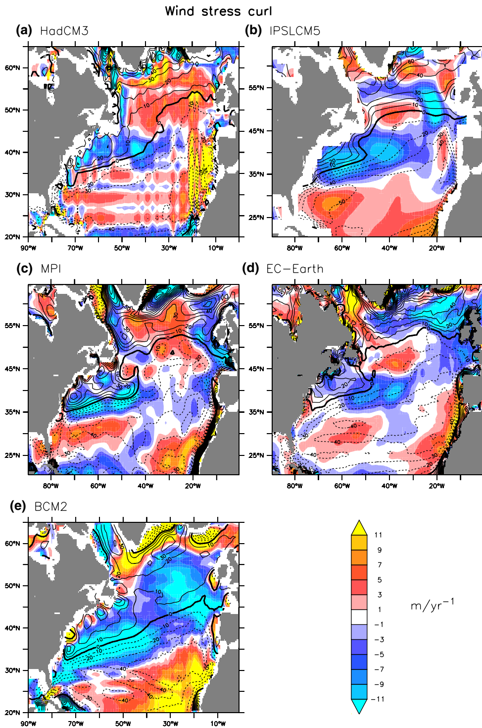
Fig. 13 Difference in wind stress curl (related to Ekman pumping) between control projection (FutCon, 2050–2089) and control historical (HisCon, 1965–2004) experiments averaged over the four decades for the different models (unit: m/year). Contoured lines are the
